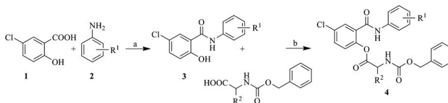
Scheme 1. Synthesis of N -protected amino acid esters. Reagents: (a) \text{PCl}_3 , chlorobenzene, microwave reactor; (b) DCC, DMF.
