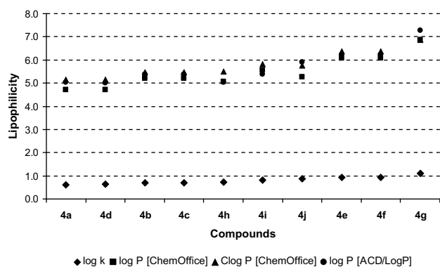
Figure 1. Comparison of \log P/\text{Clog } P data calculated using the two computer programs with the experimentally determined \log k values. The compounds are ordered according to the increase in \log k values in the series of compounds 4a–4j .
